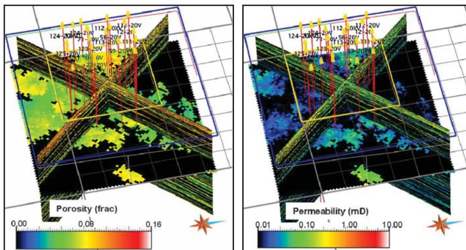
FIGURE 4 Porosity and Permeability Distributed in Pay Facies
