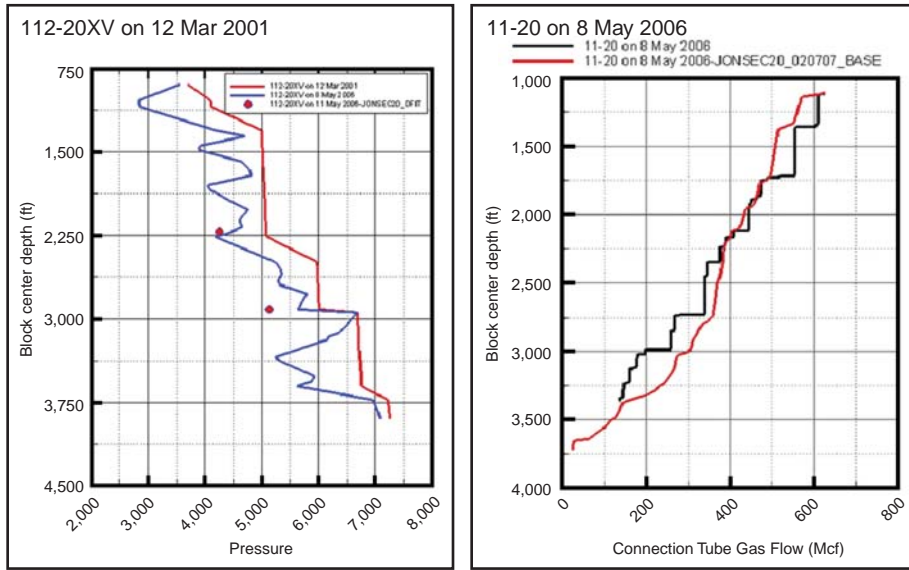
FIGURE 5 Simulated versus Measured Pressure Depletion/Production
